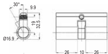
APC-AD/MB Double Key
