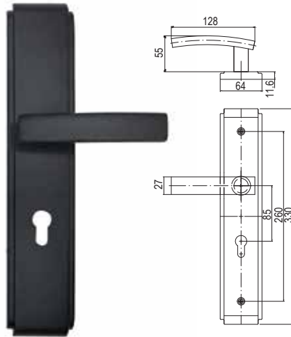
ALH-B3365/CS/MB Lever handle with plate
