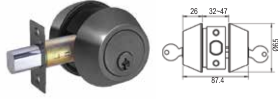
AJP-999/Matt Grey Double Cylinder Jimmy Proof Lock
