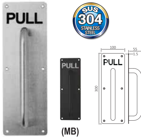
APH-PP500 Pull Plate Handle
