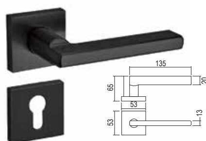
ALH-6102/MB Lever handle
