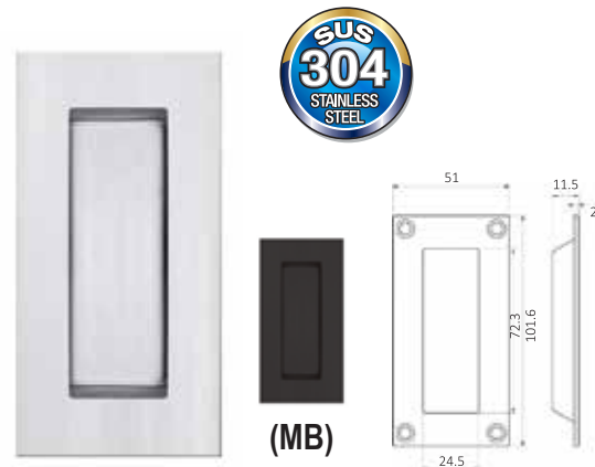
APF-42/SS Square Flush Pull
