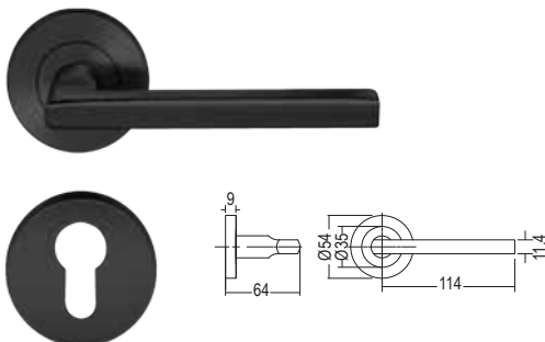
ALH-6002/MB Lever handle
