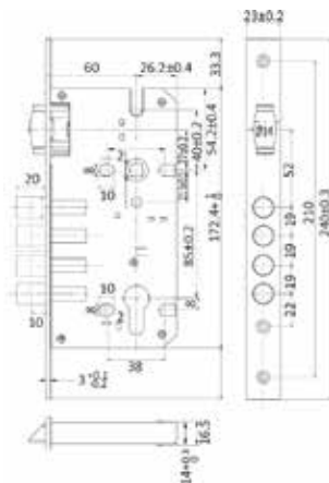
AML-A8550/MR Mortise with Four Bolts
