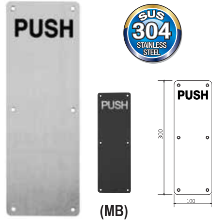
APH-PP501 Push Plate
