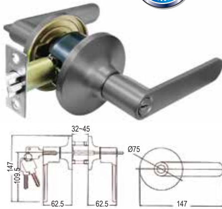
ATL-8200/Matt Grey Tubular Lever Lock
