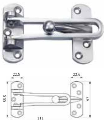
ADG-911/SN Door Guard
