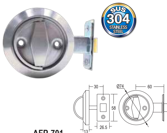
AFP-701 Flush Pull Ring
