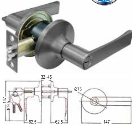
ATL-8100/Matt Grey Tubular Lever Lock
