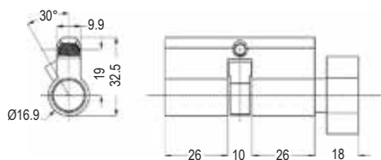
APC-AP/MB Thumbturn & Coin Slot
